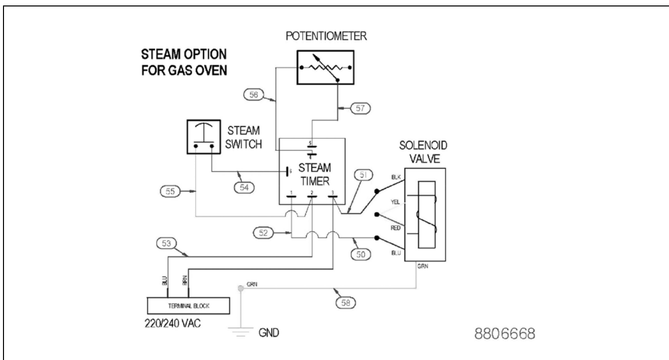
Wiring Diagram – Steam Injection 220/240V
